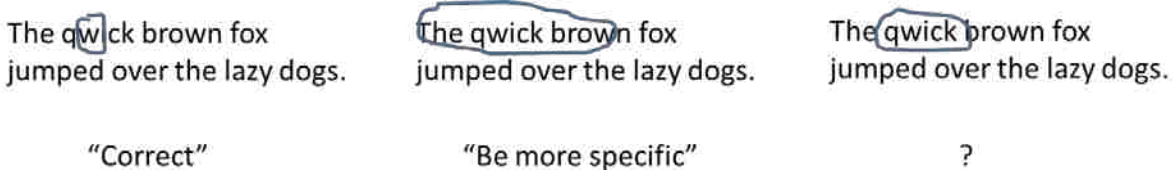
Figure 3.10: Grading Ambiguity
